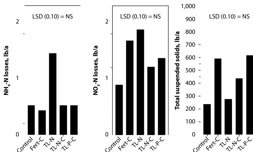
Figure 1. Two-year average NH 4 -N, NO 3 -N, and total suspended solids losses from claypan soil receiving turkey litter and/or fertilizer. Control: no fertilizer or turkey litter application with no tillage. Fert-C: commercial fertilizer only incorporated with conventional tillage. TL-N: Nitrogen-based turkey litter application with no tillage. TL-N-C: N-based turkey litter application incorporated with conventional tillage. TL-P-C: Phosphorus-based turkey litter and supplemental N application incorporated with conventional tillage.
