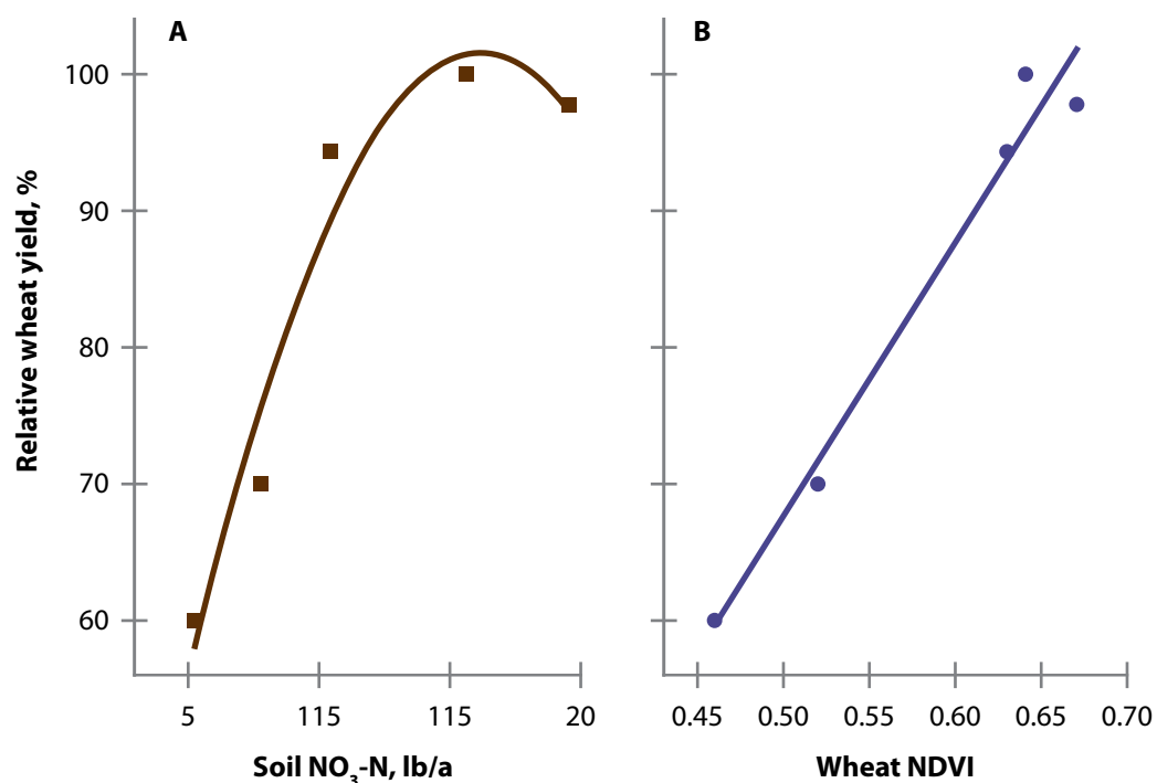
Figure 1. Effect of soil \text{NO}_3\text{-N} levels in the 0–12-in. depth and wheat normalized difference vegetative index (NDVI) readings taken at jointing (Feekes 6) on relative wheat yield in 2013.
