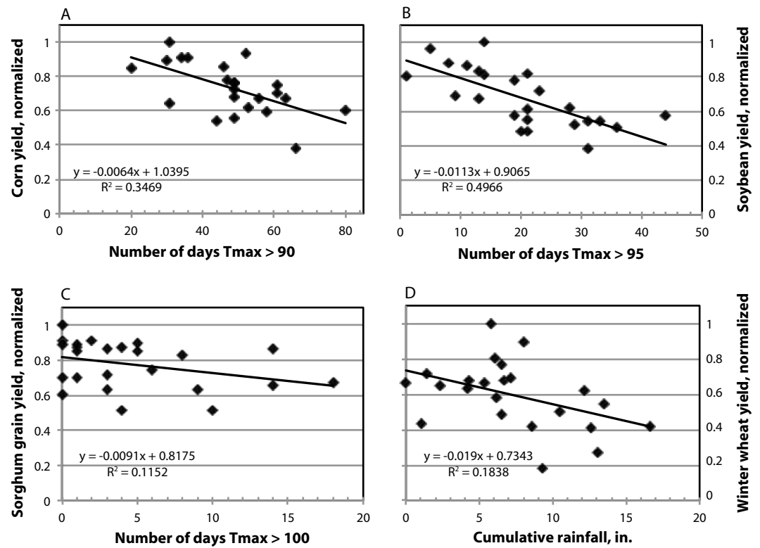
Figure 2. Correlations of crop yields to various weather parameters were calculated to better explore factors potentially affecting crop performance. Weather parameters included maximum and minimum temperature (Tmax and Tmin), rainfall, and sunlight. Cumulative rainfall was calculated over the growing season for each crop and for specific crop growth phases for winter wheat. Correlations are developed on a county level to better account for spatial variability in weather and soils. Crop yields and weather from Labette County in southeast Kansas are presented.
