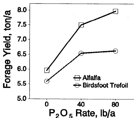
Figure 1. Effect of P Fertilization Rate on Total Forage Yield of Alfalfa and Birdsfoot Trefoil in 1992.
