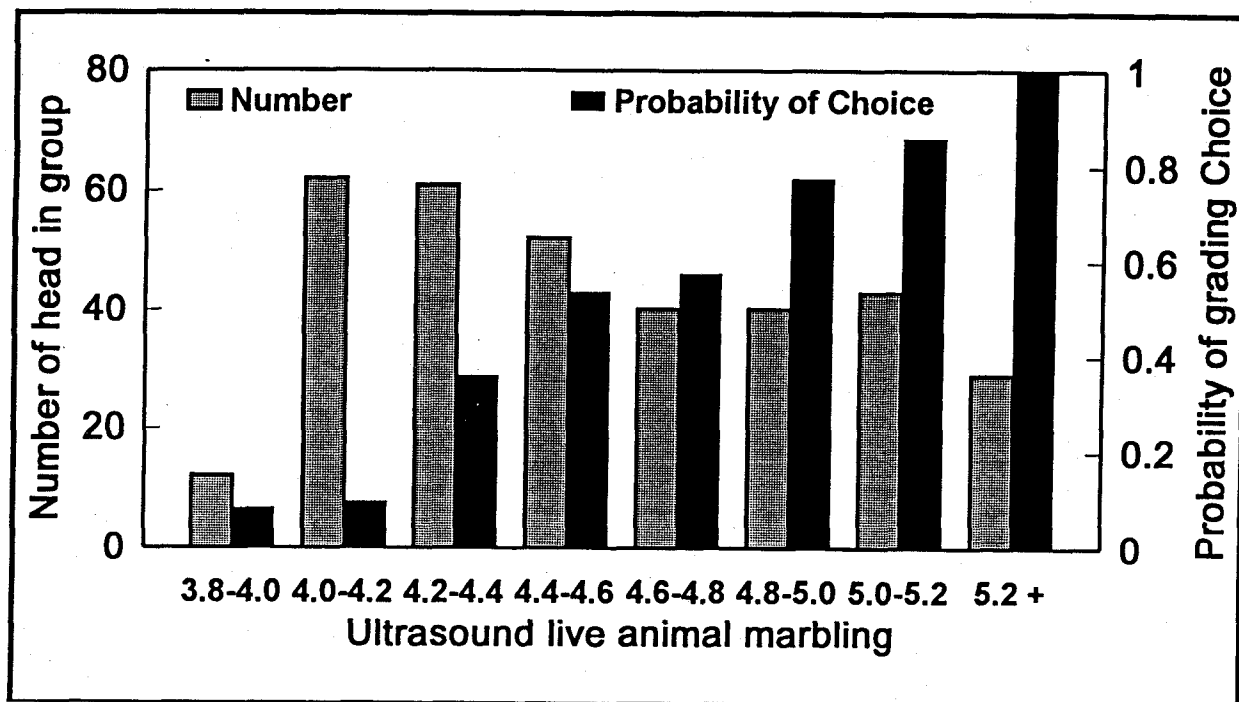
Figure 2. Relationship of ultrasound marbling estimate and likelihood of carcass grading USDA Choice 47 days later.
