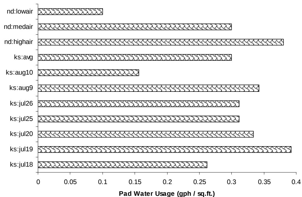
Figure 4. Comparison of Evaporative Pad Water Usage during All of the Monitoring Periods at the KS and ND Dairies.
