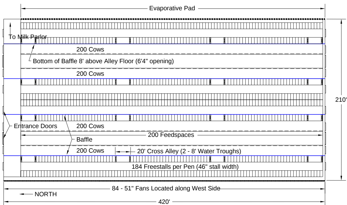
Figure 3. Top View of a Typical Layout of an 8-row Low-profile Cross-ventilated Freestall Building. The building length is adjustable on the basis of cow numbers.
