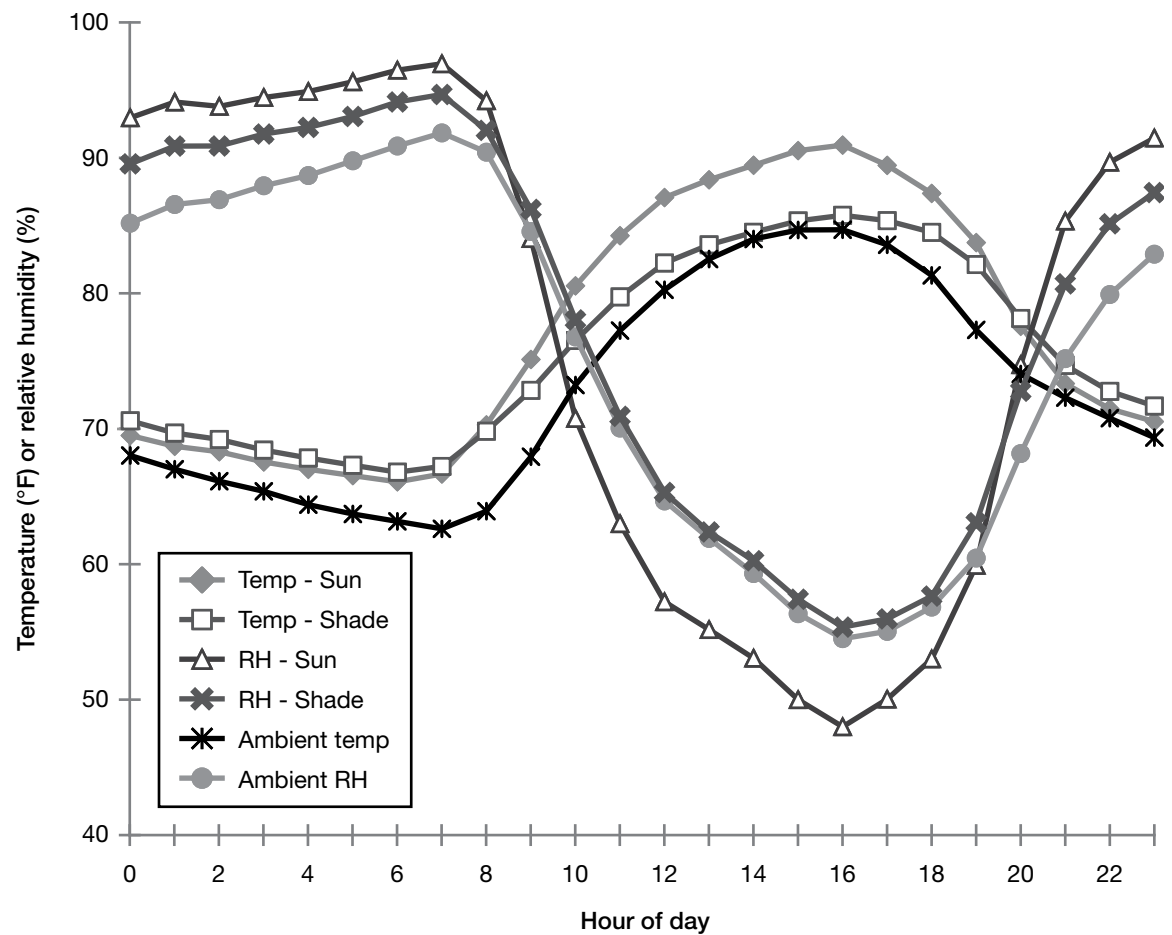
Figure 7. Average calf hutch temperature and relative humidity (July 27 to August 30, 2008).
