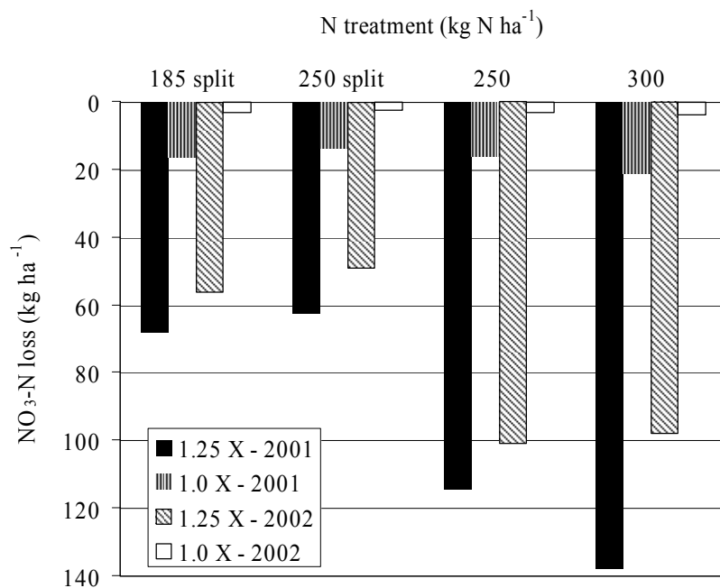
Figure 5. Total NO 3 -N flux at the 60-inch depth during the growing season. Determined by multiplying NO 3 -N concentration by average water flux between sampling dates.
