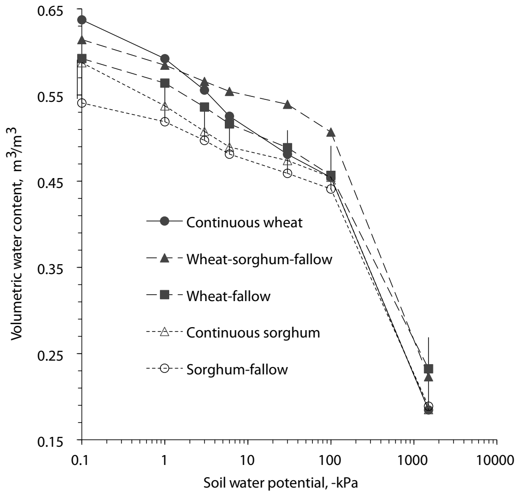
Figure 2. Soil water characteristics curve for five cropping systems under no-till for the 0- to 3-in. soil depth.
