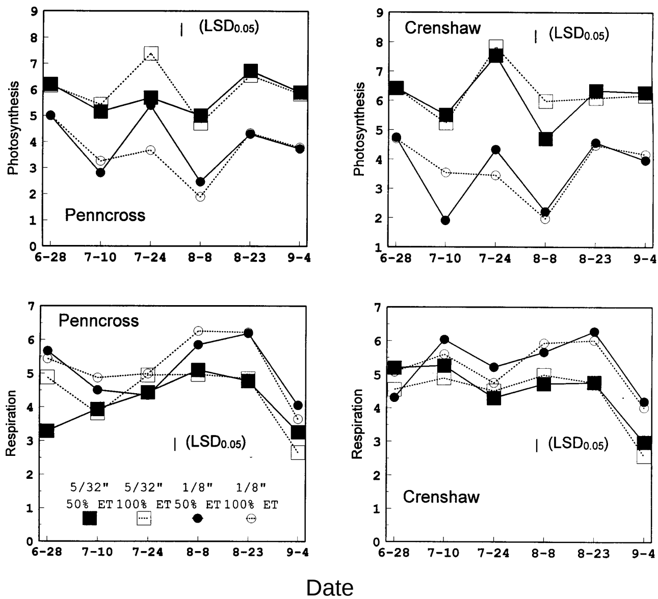
Figure 4. Effects of mowing height and irrigation on photosynthesis and respiration rate of bentgrass.
