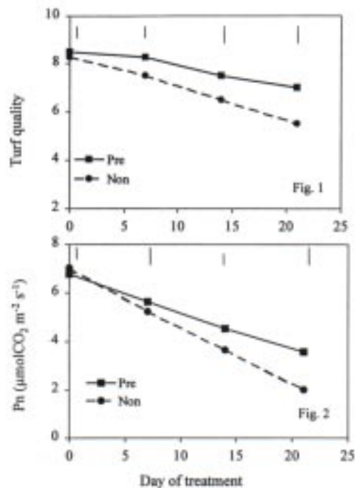
Fig.1.Turf quality and Fig.2. canopy photosynthetic rate (Pn) as affected by heat stress in drought-preconditioned (pre) and non-preconditioned (non) Kentucky bluegrass. Vertical bars indicate LSD values ( p=0.05 ) for treatment comparison at a given day of treatment.
