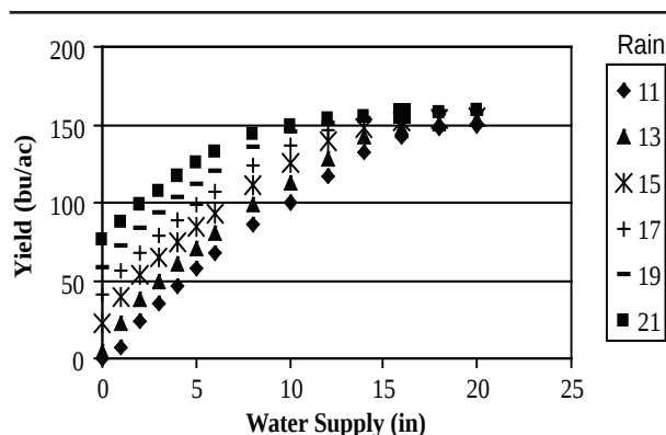
Figure 1. Yield-irrigation relationship for grain sorghum, with annual rainfall from 11 to 21 inches.
