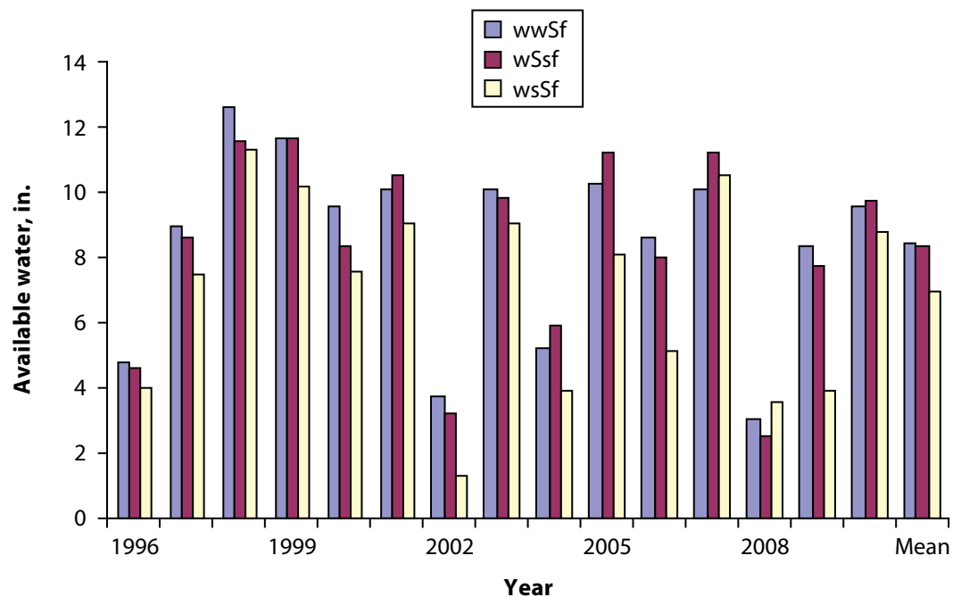
Figure 2. Available soil water at planting of sorghum in several rotations, Tribune, 1996–2010.
