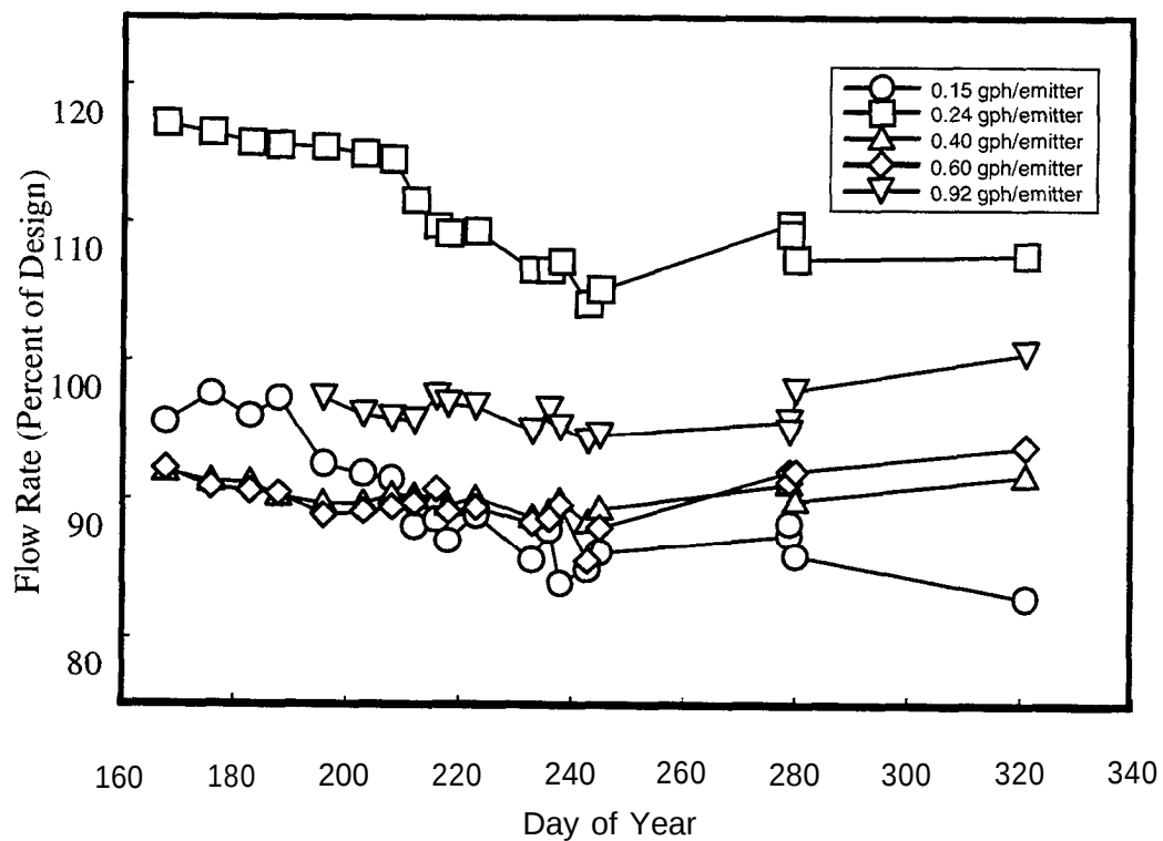
Figure 1. Measured flow rates for five dripline types in a subsurface drip-irrigation system using livestock wastewater, Midwest Feeders, Ingalls, KS, 1998.
