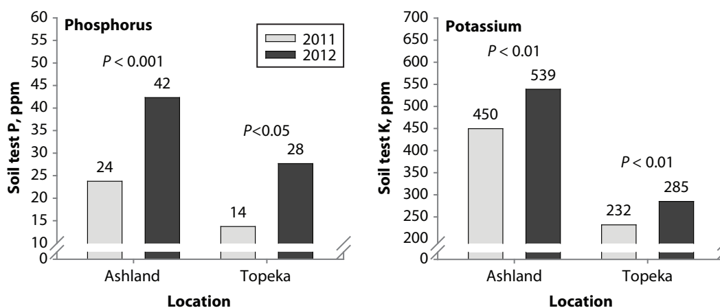
Figure 1. Soil test phosphorus (Mehlich-3) and potassium (ammonium acetate) levels as affected by fertilizer application of 120 lb/a P_2O_5 (20 lb/a P_2O_5 as starter and 100 lb/a P_2O_5 as broadcast) and 120 lb/a K_2O (20 lb/a K_2O as starter and 100 lb/a K_2O as broadcast) in 2012 after 1 year of fertilizer application on non-fertilized plots from 2011.
