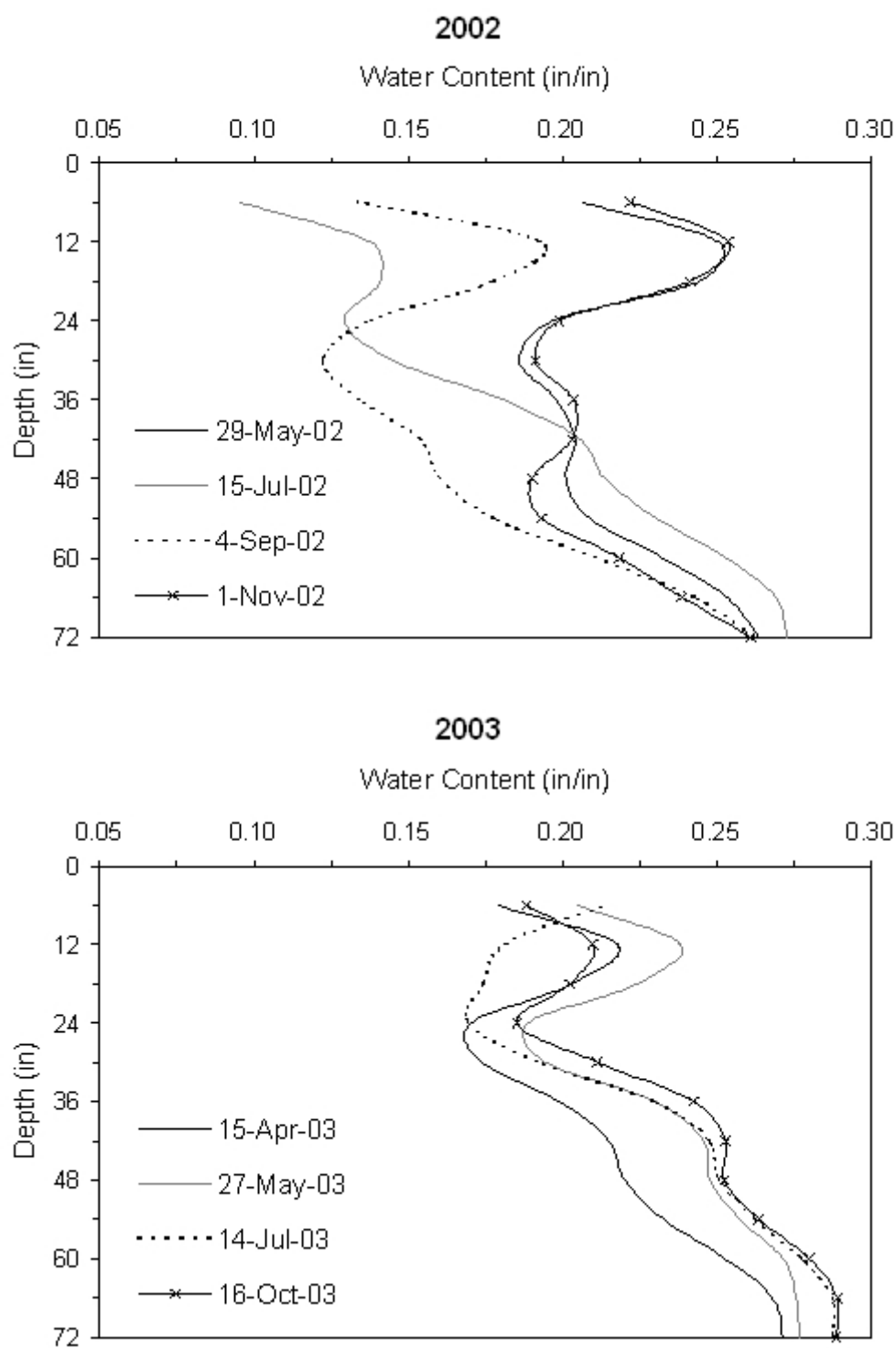
Figure 5. Water content profiles near Scandia, KS (2002 and 2003).
